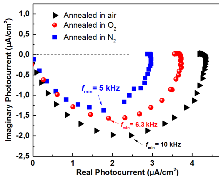
Figure 7. IMPS data of ALD \text{WO}_3 films annealed in different atmospheres (applied potential: 1.23 V vs. RHE; frequency range: 10^{-1} to 10^5 Hz).
