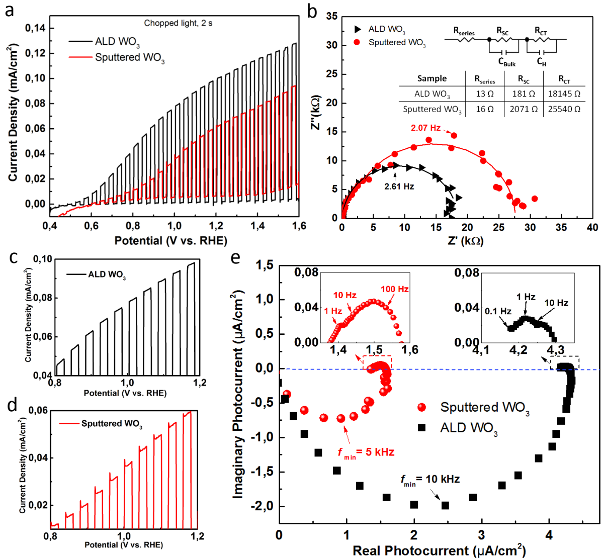
Figure 4. PEC characterization of ALD (black) and sputtered (red) WO_3 thin films: (a) Photocurrent density vs. applied potential curves under chopped light illumination (2 s light on and off, respectively). (b) Nyquist plots of the measured (dots) and fitted (line) impedance spectra at an applied potential of 1 V vs. RHE in the frequency range of 10^{-1} to 3 \times 10^5 Hz; insets are the equivalent circuit model and the fitting values of R_{series} , R_{SC} and R_{CT} ; (c) and (d) are enlargements of the light-on part of the curves in (a) at 0.8 V to 1.2 V vs. RHE; (e) IMPS data at an applied potential of 1.23 V vs. RHE in the frequency range of 10^{-1} to 10^5 Hz (insets: enlargement of the plot in the first quadrant).
