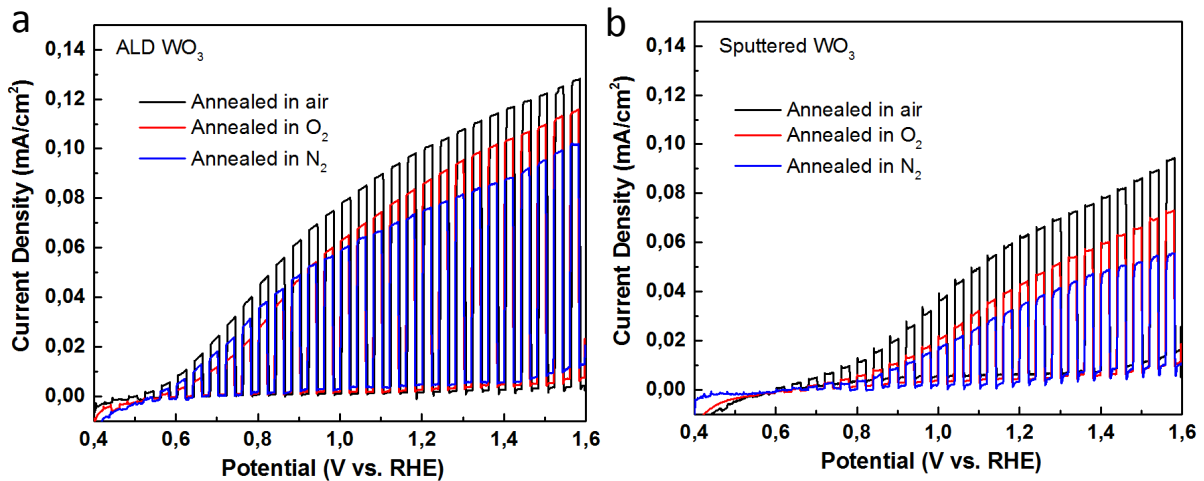
Figure 6. Photocurrent density vs. applied potential of (a) ALD and (b) sputtered \text{WO}_3 films annealed in different atmospheres (chopped light measurements with t = 2\text{ s} ).
